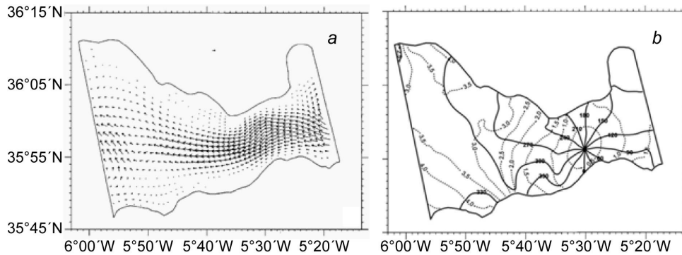
Fig. 2. a — M_2 tidal energy flux; b — O_1 cotidal chart.
