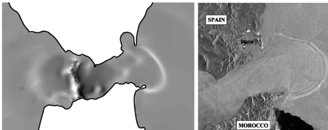
Fig. 3. Spatial structure of internal bore in the Strait of Gibraltar. The left panel shows the model predictions of the surface strain. The right panel is an ERS-1 SAR image (6-Feb-1992, 1104 UTC, orbit 2929, frames 2871/2889) of surface signatures of an eastward-travelling internal bore. Lighter shading shows the bore front.
