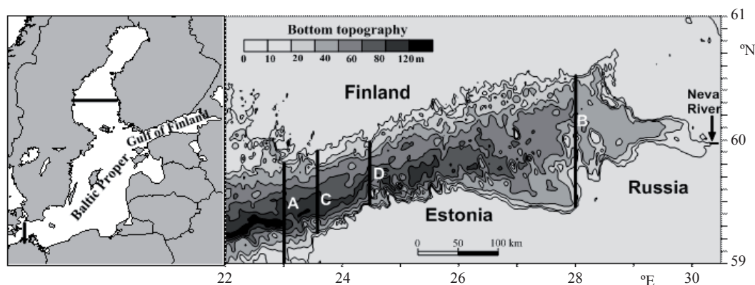
Fig. 1. A map of the Baltic Sea (left panel) and Gulf of Finland (right panel).
