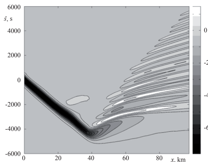
Fig. 9. Contour plot in the space-time domain of an ISW along cross-section 1. The displacement (m) of an isopycnal at the position of maximum of the first vertical linear baroclinic mode is shown.
