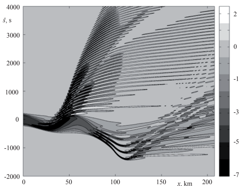
Fig. 15. Contour plot in the space-time domain of an ISW along cross-section 2. The displacement (m) of an isopycnal at the position of maximum of the first vertical linear baroclinic mode is shown.
