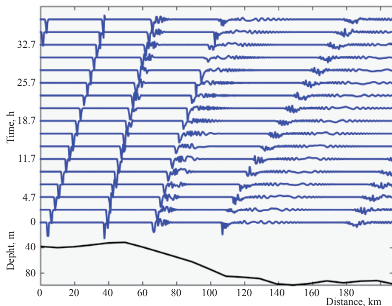
Fig. 17. Transformation of an ISW along cross-section 2. The displacement (m) of an isopycnal at the position of maximum of the first vertical linear baroclinic mode is shown. The vertical shift between successive curves is 5 m.
