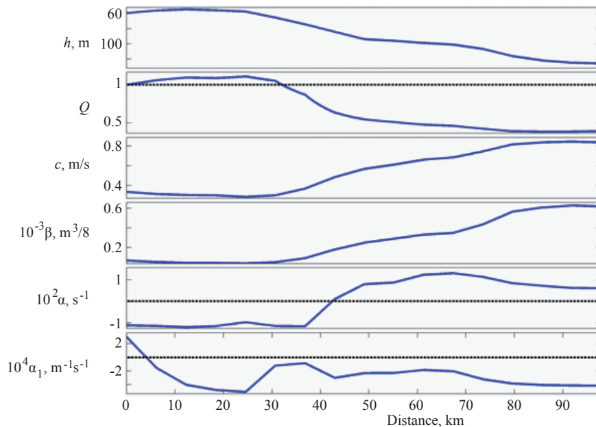
Fig. 8. Coefficients of the variable-coefficient Gardner's equation along cross-section 1.
