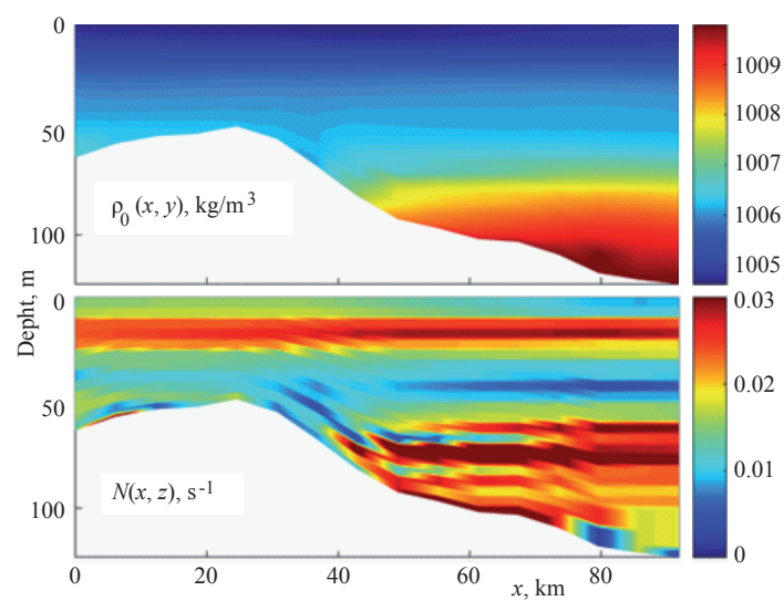
Fig. 7. Undisturbed sea water density and Brunt-Väisälä frequency along cross-section 1.
