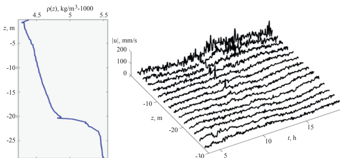
Fig. 5. Density profile (left) and records of the absolute value of horizontal velocity (right) on 16 June 2010 near the coast of the Curonian Spit in the south-eastern part of the Baltic Sea [25].
