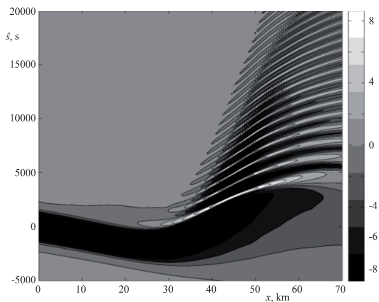
Fig. 16. Contour plot in the space-time domain of an ISW along cross-section 3. The displacement (m) of an isopycnal at the position of maximum of the first vertical linear baroclinic mode is shown.
