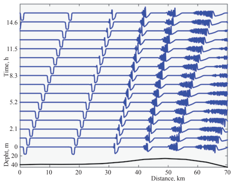
Fig. 18. Transformation of an ISW along cross-section 3. The displacement (m) of an isopycnal at the position of maximum of the first vertical linear baroclinic mode is shown. The vertical shift between successive curves is 10 m.
