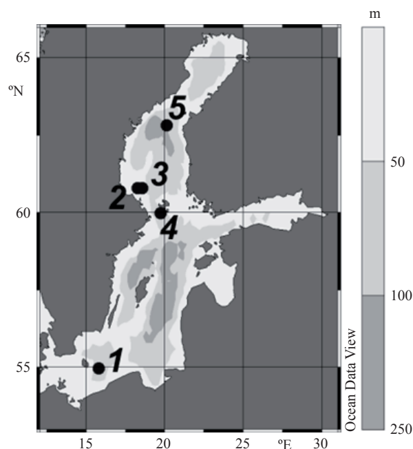
Fig. 1. Locations of observations 1—5 (table) of surface manifestations of IWs on satellite SAR images of the Baltic Sea on the background of bathymetry.
