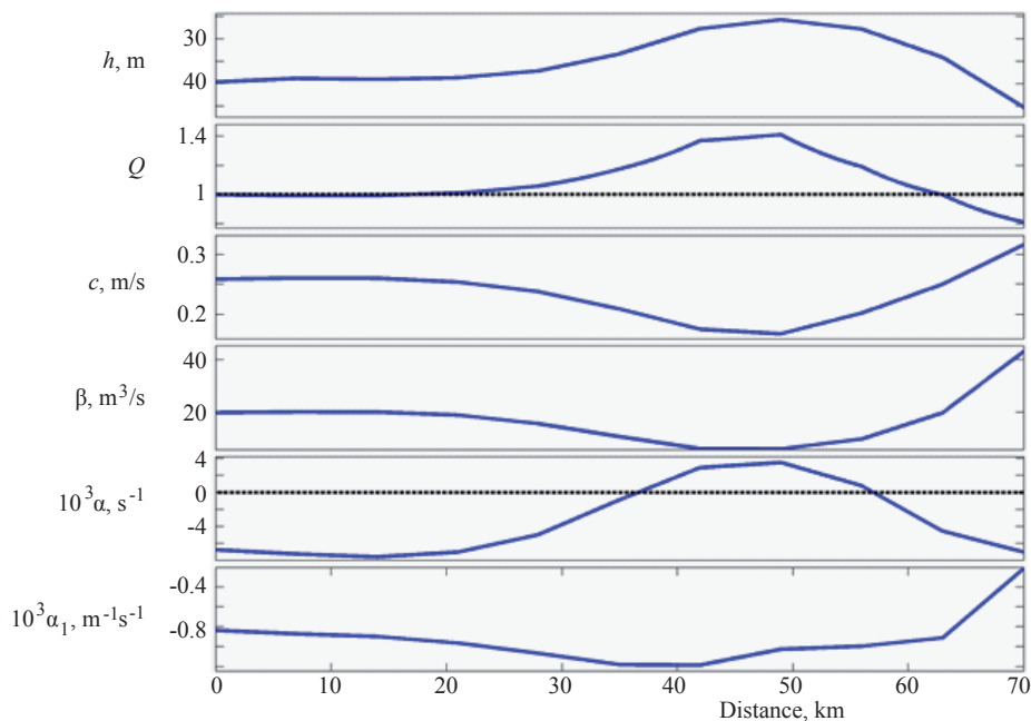
Fig. 14. Coefficients of the generalized Gardner's equation along cross-section 3.
