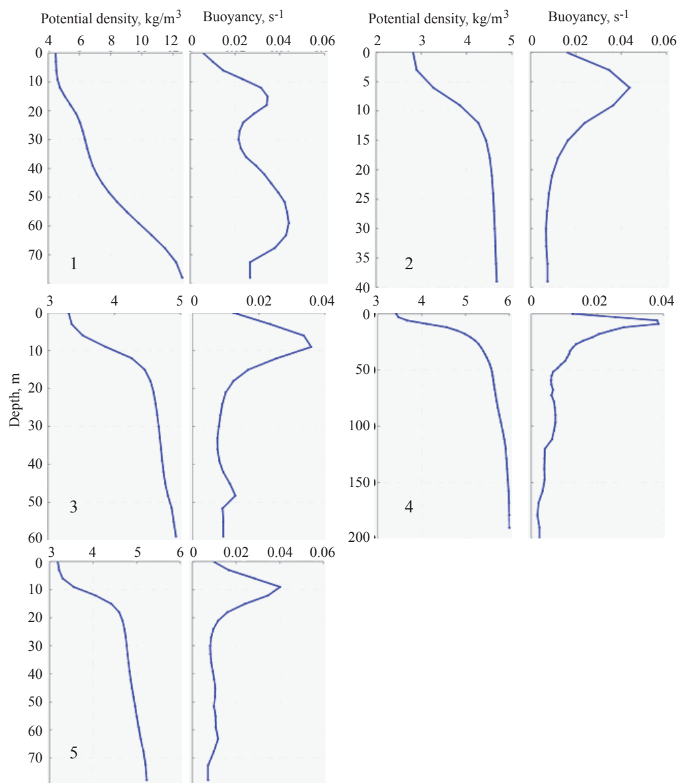
Fig. 3. Density and buoyancy profiles for the locations in the Table.
