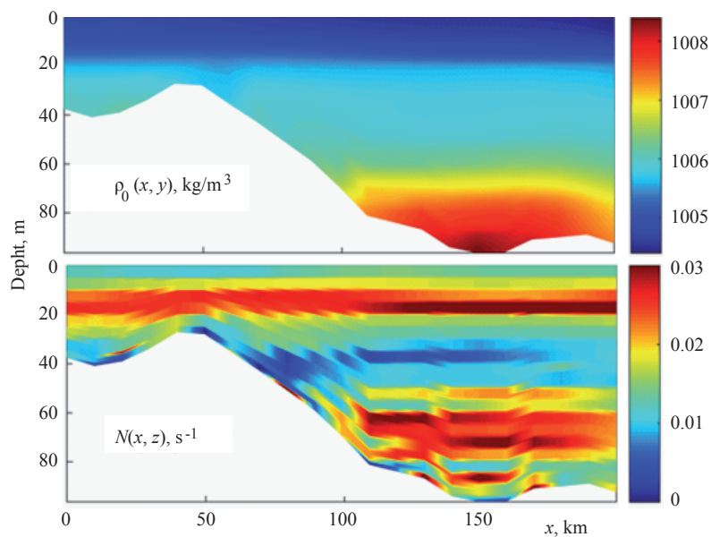
Fig. 11. Undisturbed sea water density and Brunt–Väisälä frequency along cross-section 2.
