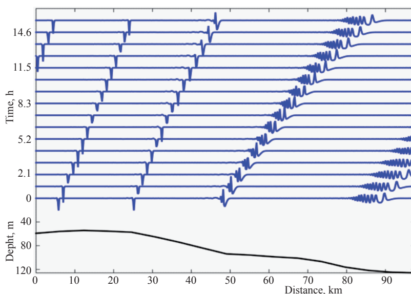
Fig. 10. Transformation of an ISW along cross-section 1. The displacement (m) of an isopycnal at the position of maximum of the first vertical linear baroclinic mode is shown. The vertical shift between successive curves is 5 m.
