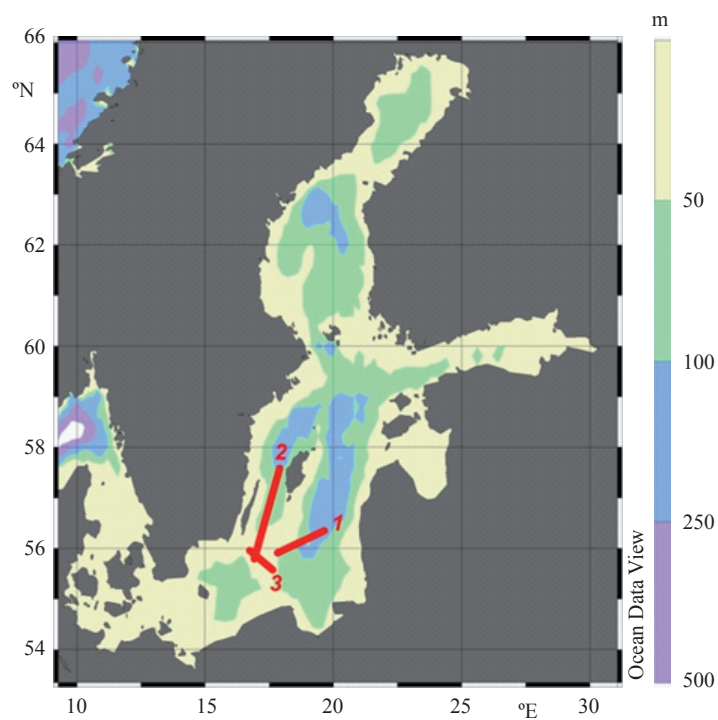
Fig. 6. Bathymetry of the Baltic Sea, with the chosen cross-sections.
