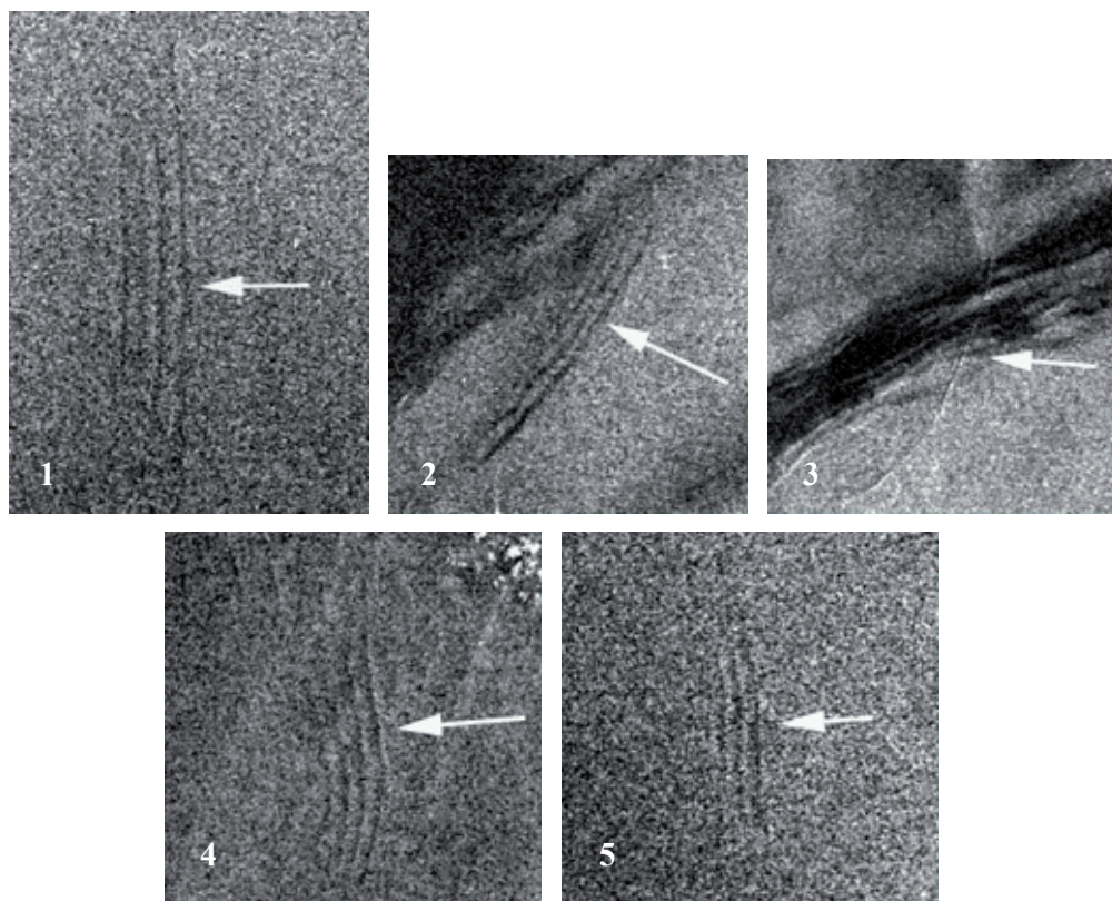
Fig. 2. Surface manifestations of IWs (subimages of Envisat ASAR images from http://www.iki.rssi.ru/asp/iw_images/index.html ) in the Table.
