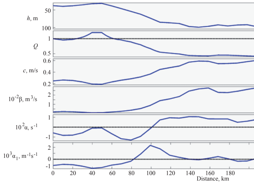
Fig. 12. Coefficients of the variable-coefficient Gardner's equation along cross-section 2.
