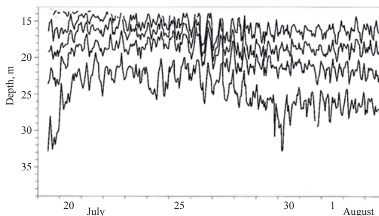
Fig. 4. Isotherms for a 16-day period in July—August 1978 in the Sea of Bothnia [10].
