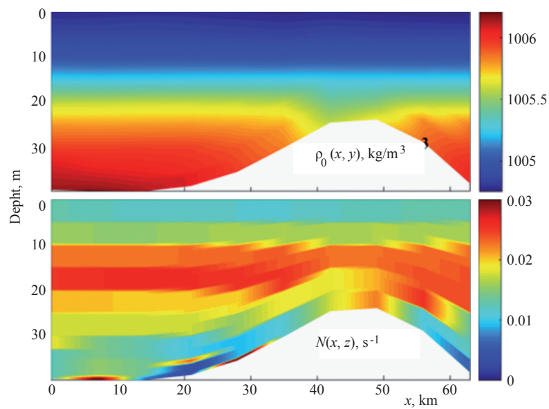
Fig. 13. Undisturbed sea water density and Brunt–Väisälä frequency along cross-section 3.
